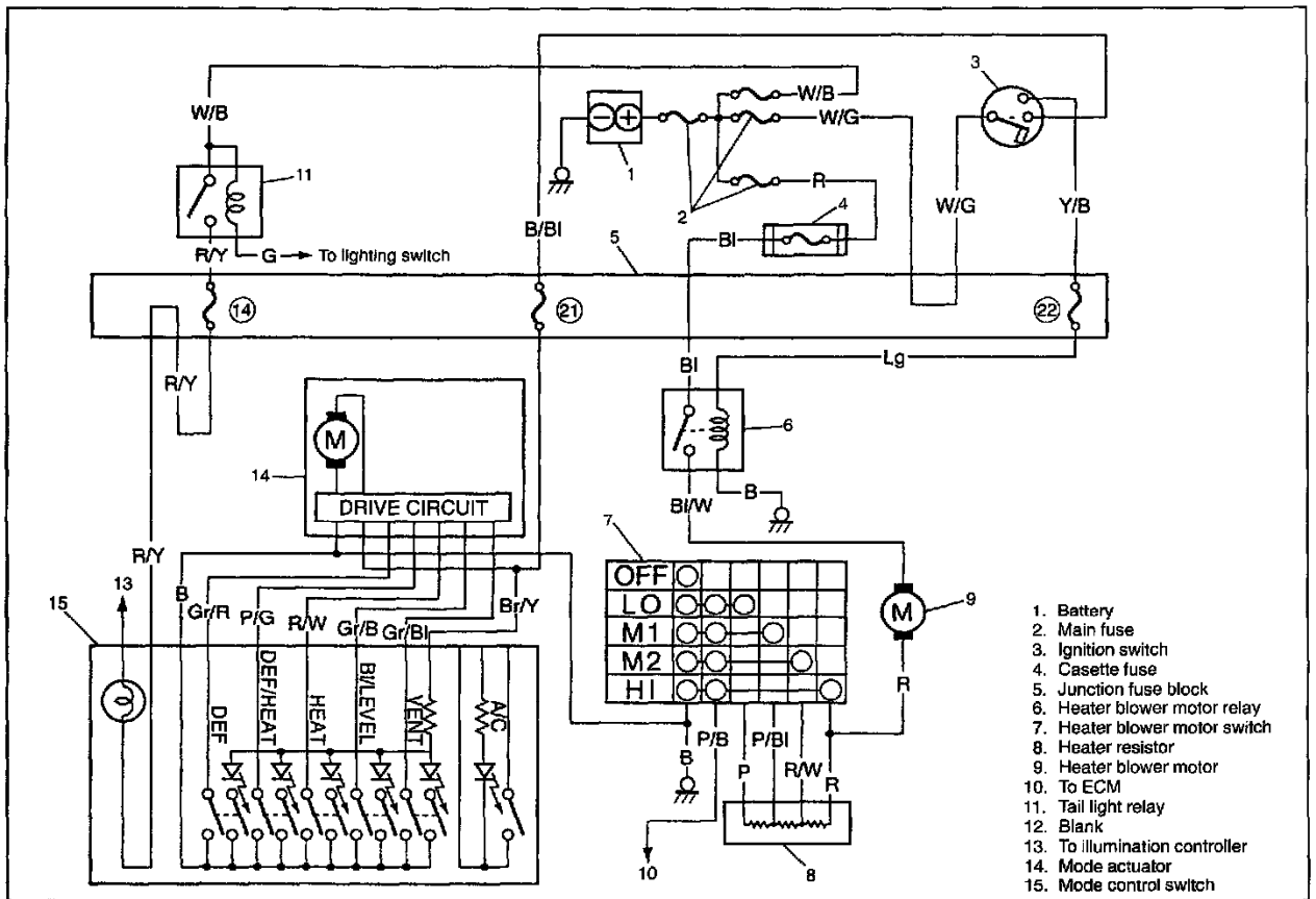
Wiring Circuit
